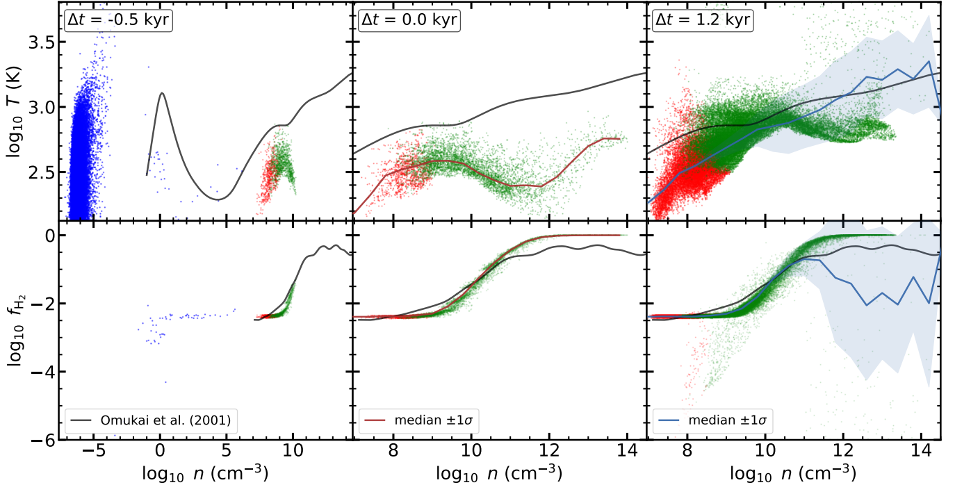
FIG. 3.— Phase diagram (temperature and H_2 fraction vs. number density) at three representative epochs: pre-stellar ( t - t_1 \approx -0.5 kyr, left), first sink formation ( t - t_1 = 0 , middle), and post-first-sink ( t - t_1 = 1.2 kyr, right). Green points correspond to disk-identified particles, red points correspond to points in our cutout simulation that have not been identified as disk, and blue points correspond to points in the full-box simulation right before the cutout was applied (only included in the leftmost plots). f_{H_2} = 0 for most of particles in the low-density region (blue particles), thus missing from the bottom-left panel. Solid black curves show the zero-metallicity Population III collapse track (Omukai (2000), as digitized by Klessen and Glover (2023)) on the temperature (top) and H_2 fraction (bottom) panels. Coloured curves with shaded bands are binned medians of the simulated gas (the bands span \pm 1\sigma ): blue is the instantaneous median at the pre-stellar epoch; dark red is the mean of the per-snapshot medians over -0.5 \text{ kyr} \leq t - t_1 \leq 0 , and dark blue over 0 \leq t - t_1 \leq 1.2 \text{ kyr} .
