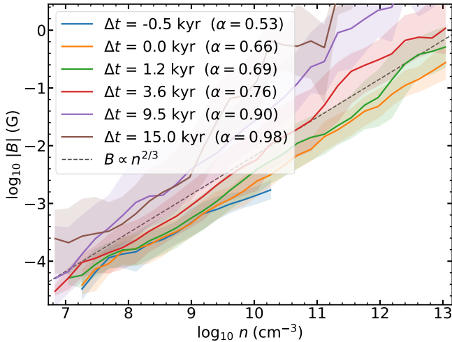
FIG. 13.— Evolution of phase plot of magnitude of magnetic field |B| vs number density n . Solid lines correspond to median profiles at different times, with the shaded regions being 90-th percentile of all the particles. \alpha corresponds to the exponent in power-law fit |B| \propto n^\alpha . |B| spans 3 orders of magnitude at the point of first sink formation, and up to 4 orders of magnitude at later times. [SK: Fix this figure]
