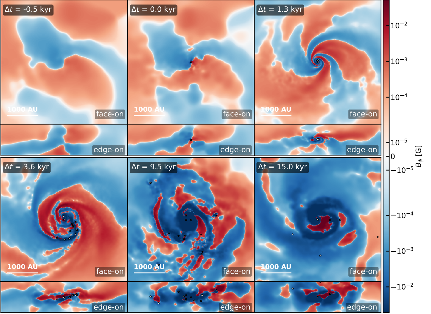
FIG. 11.— Face-on ( z = 0 slice) and edge-on ( x = 0 slice) of the toroidal magnetic field component B_\phi at six epochs.
