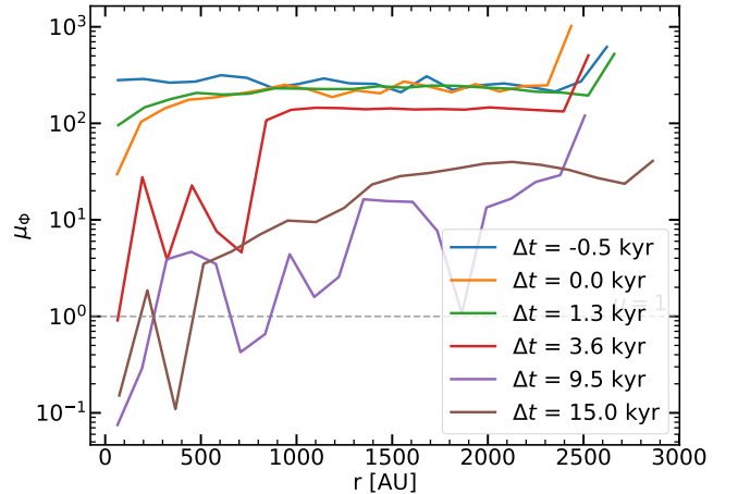
FIG. 14.— Dimensionless mass-to-flux ratio \mu_\Phi as a function of radius at six epochs. The dashed line marks the critical value \mu_\Phi = 1 . The disk evolves from highly supercritical ( \mu_\Phi \sim 100-300 ) at early times to partially subcritical ( \mu_\Phi < 1 ) at some inner radii by 9.5 kyr.
