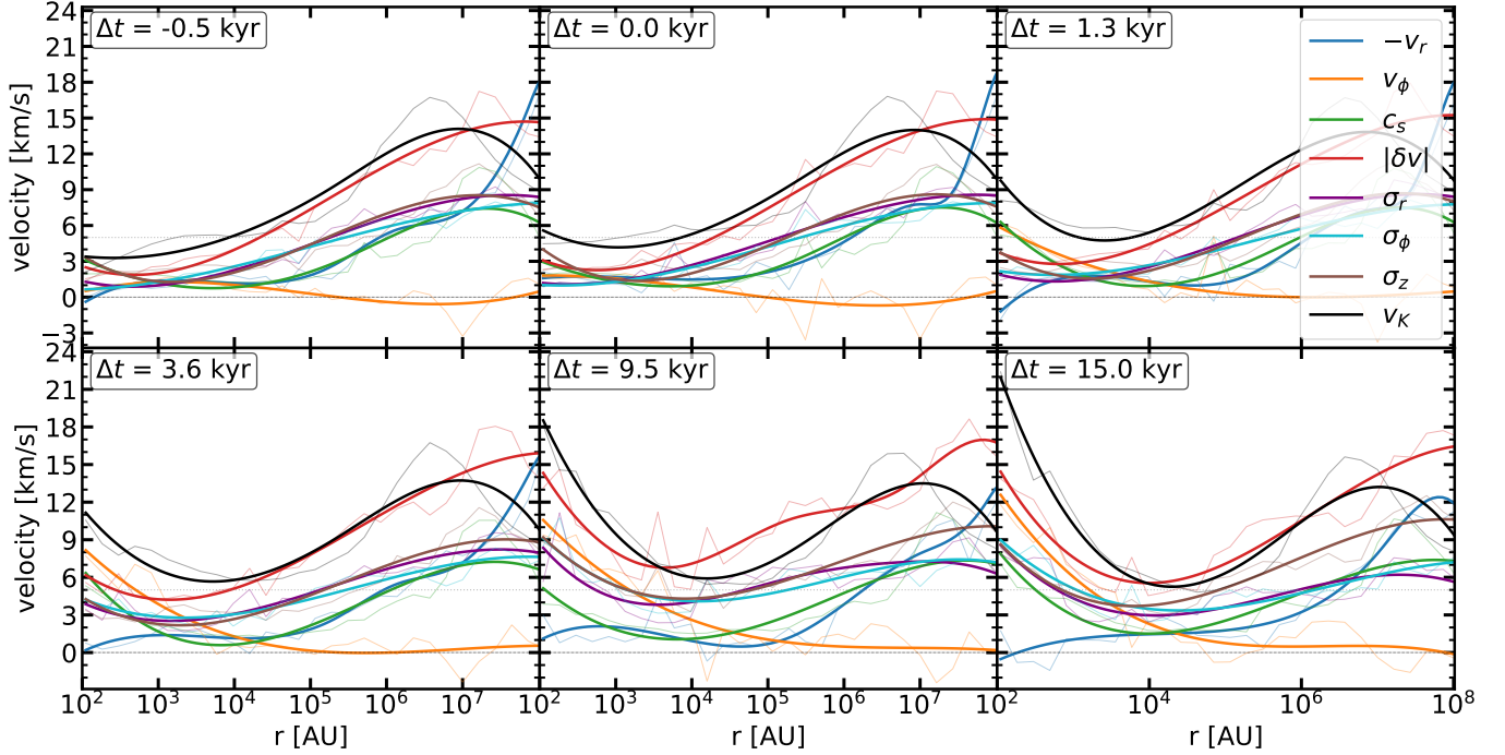
FIG. 7.— Radial profiles of inward radial velocity -v_r , azimuthal velocity v_\phi , sound speed c_s , magnitude of turbulent velocity |\delta v| , radial/azimuthal/vertical turbulent velocity dispersion \sigma_r/\sigma_\phi/\sigma_z , Keplerian speed v_K of gas particles in the disks. Bright lines show functions with spline smoothing, dim lines show actual data. \sigma_r grows with time, as well as |\delta v| . Radial infall ( v_r ) speeds up until the bulk star formation events (1.3–3.6 kyr), and slows down afterwards. Disk rotation ( v_\phi ) is constantly speeding up, leveling off outside of the disk ( r \gtrsim 2500 AU). \sigma_r, \sigma_\phi, \sigma_z track each other very closely, but \sigma_z decouples from the other two by the \Delta t \gtrsim 9 kyr time outside of the disk. Turbulence is supersonic at all times, tracking Keplerian speed v_K closely for most times outside of the disk, but falling below it inside of the disk.
