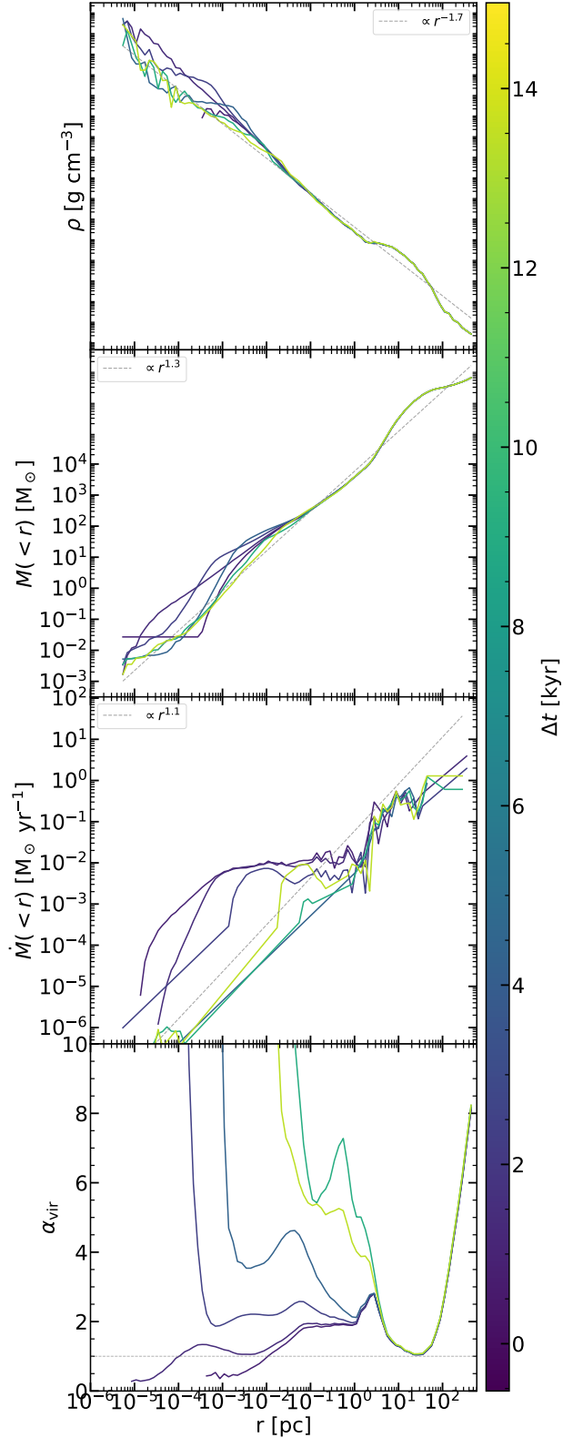
FIG. 5.— First plot: Radial density profiles through simulation time. The x-axis begins at \sim 1 AU, corresponding to the resolution limit of the simulation. The fit for the region outside of the disk is consistently \rho \propto r^{-1.7} across all times. Second plot: Gas mass in a ball vs radius of the ball before the formation of the first sink. The fit is roughly M \propto r^{1.3} . Third plot: rate of change of the gas mass enclosed within a sphere of radius r , i.e. the integrated “mass of the ball” accretion rate \dot{M}(< r) = dM(< r)/dt . At later times the inner region gains mass slower than at the earlier times (mostly close to the time of the first sink forming). There is a characteristic “flattening” at smaller radii inside of the disk before the first star has formed. Outer shells gain mass faster at all times – a characteristic of “outside-in” collapse. Smallest shells have a drop in \dot{M}(< r) , associated with coming close to the resolution limit.
