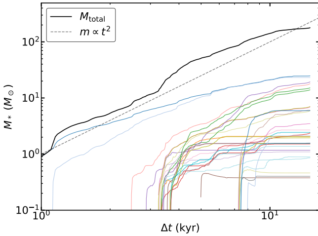
FIG. 16.— Evolution of masses of individual sinks. Dashed line represents ideal M_* \propto t^2 law, which is being followed for total mass of all the sinks (black line). At earlier times, before the first bulk star formation event at 2–3 kyr, all of stellar mass is concentrated in the 2 central sinks (top blue lines). These massive sinks reach mass of around 20M_\odot by the 15 kyr mark, with their accretion slowing down compared to less massive sinks, which still accrete rapidly.
