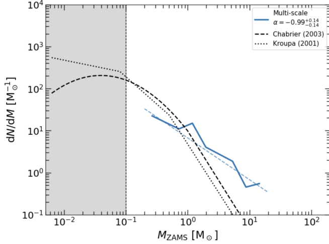
FIG. 19.— Protostellar mass function at t - t_1 = 15 kyr (blue solid histogram) compared to the Chabrier (2003) (dashed) and Kroupa (2001) (dotted) present-day IMFs. The best-fit high-mass power-law slope is \alpha = -0.99^{+0.14}_{-0.14} (light blue dashed line), shallower than but comparable to the Salpeter slope ( -2.35 ). The grey shaded region marks masses below the completeness limit of the simulation. As this is a initial mass function measured at 15 kyr, the final masses will be modified by continued accretion, mergers, ejections, and radiative feedback.
