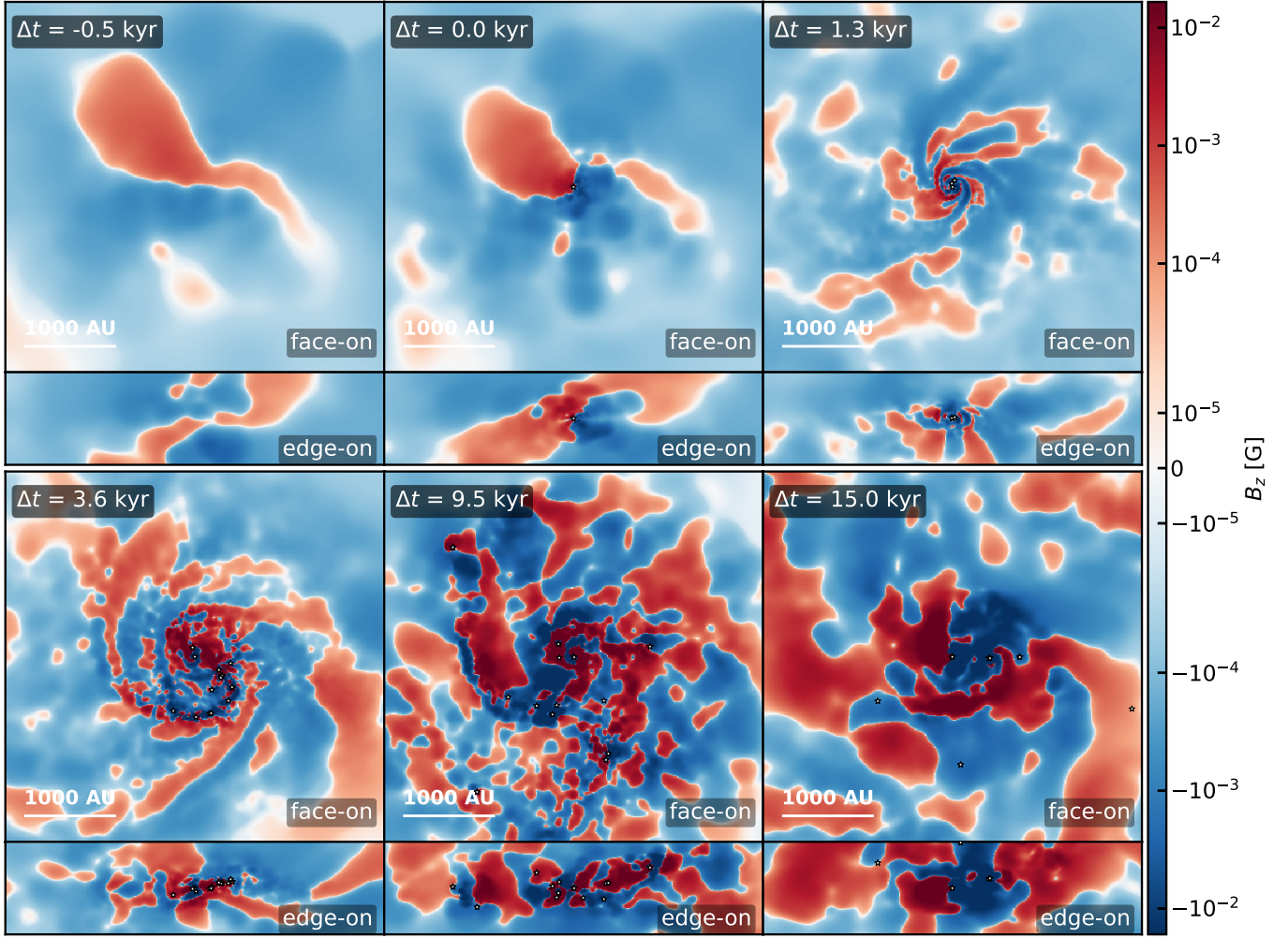
FIG. 12.— Face-on ( z = 0 slice) and edge-on ( x = 0 slice) of the vertical magnetic field component B_z at six epochs. By the late epochs shown here, most of the stars in the simulation have already formed, so the field structure reflects the post-formation disk rather than the initial collapse.
