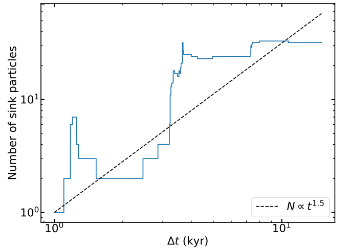
FIG. 18.— Time evolution of the number of sinks in the simulation. The dashed line shows a N \propto t^{1.5} power law for comparison (Li et al. 2018). Bulk star formation events in the spiral arms (visible in the bottom panels of Figure 9) are seen to rapidly increase the number of sinks at t - t_1 \approx 3 –4 kyr and 7–8 kyr.
