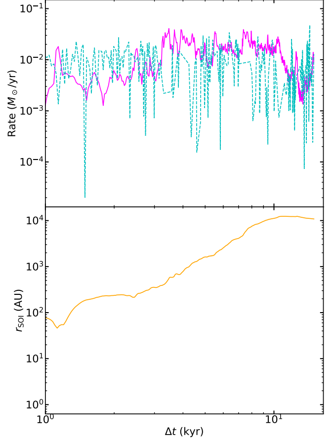
FIG. 17.— Top: stellar accretion rate (magenta) and gas depletion rate within the aperture (cyan dashed). Bottom: sphere of influence radius r_{\text{SOI}} ( M_{\text{gas,enc}} = M_* ; orange), growing from \sim 80 AU to \sim 10^4 AU over the simulation.
