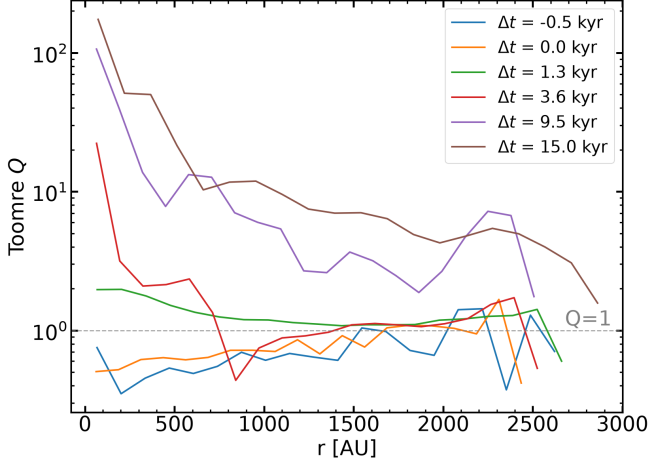
FIG. 10.— Toomre Q radial profiles time evolution. The disk starts with Q < 1 inside and Q \approx 1 near the edge, but Q rises with disk evolution, since gas is removed from the disk because of star formation events. Center of the disk is extremely stable ( Q \gtrsim 10^2 ) by the 15 kyr mark, preventing any further star formation in the middle. [SK: I don't think this plot adds any new information, you can get rid of it to keep things more concise.]
