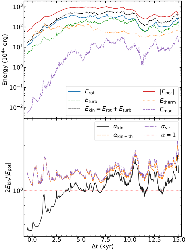
FIG. 4.— Top: Time evolution of the main energy components computed for disk-identified particles (the disk radius r_{\text{disk}} is taken as the 90th-percentile cylindrical radius of disk-identified particles, see subsection 3.2): rotational kinetic energy E_{\text{rot}} (blue), turbulent kinetic energy E_{\text{turb}} (green), total kinetic energy E_{\text{kin}} = E_{\text{rot}} + E_{\text{turb}} (black, dash-dotted), gravitational potential energy |E_{\text{pot}}| (red), thermal energy E_{\text{therm}} (orange, dotted), and magnetic energy E_{\text{mag}} (magenta, dashed). Bottom: pure kinematic virial ratio \alpha_{\text{kin}} = 2E_{\text{kin}}/|E_{\text{pot}}| (black); virial ratio with added thermal component \alpha_{\text{kin+th}} = 2(E_{\text{kin}} + E_{\text{therm}})/|E_{\text{pot}}| , and with added thermal and magnetic components (purple, dash-dotted), \alpha_{\text{vir}} = 2(E_{\text{kin}} + E_{\text{therm}} + E_{\text{mag}})/|E_{\text{pot}}| . The dotted red line marks virial equilibrium ( = 1 ). The disk starts sub-virial and reaches equilibrium by \sim 2 kyr. The inclusion of thermal energy reveals that the disk is thermally supported and near virial equilibrium at all times. Magnetic energy provides negligible additional support to the virial ratio.
